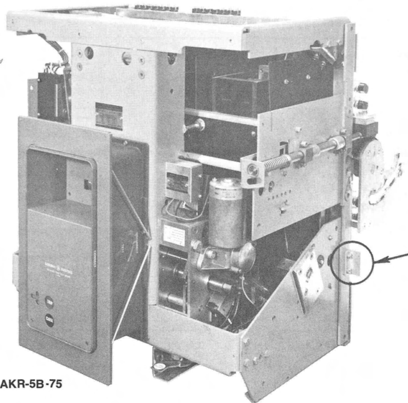
Fig. 14 Rejection means on AKR-75/100 code B, D and F type drawout breakers to exclude them from AKD type compartments.
