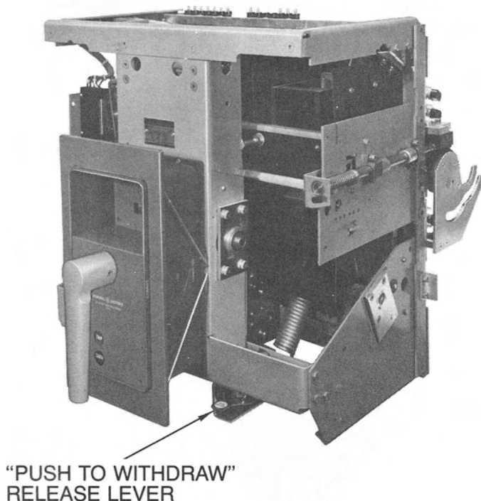
Fig. 4 AKR-5B-75 manually operated (substructure type)
