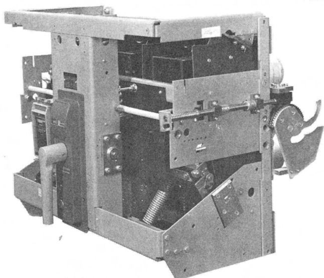
AKR-5-100 Manually operated, AKD type
