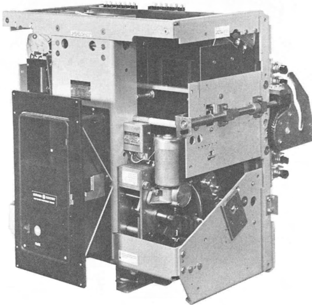
FIG. 6 AKR-6D-75 ELECTRICALLY OPERATED (AKD-8-TYPE)
