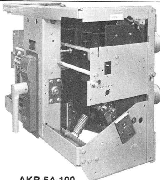
AKR-5A-100 Manually operated, AKD-5 type
