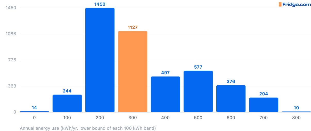
Distribution of certified annual energy use
